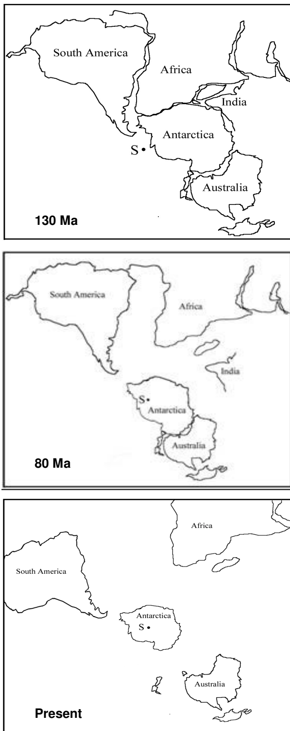
Figure 2: The break-up of Gondwanaland, the southern hemisphere super-continent formed by the union of proto-Australia, Antarctica, South America, Africa and India and associated islands (e.g. New Guinea, New Zealand and Madagascar). Separation started around 100 million years ago (Ma) and by 80Ma only Australia and Antarctica were still connected. Adapted from Smith and Briden (1977).
